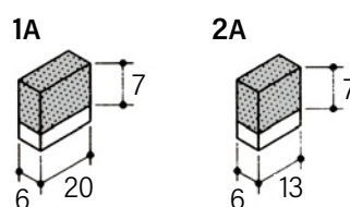
鑽石齒塊尺寸 / The dimensions of diamond tips
