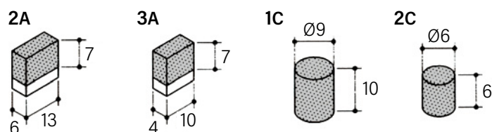
鑽石齒塊尺寸 / The dimensions of diamond tips
