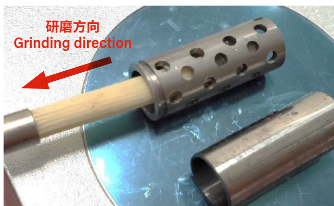
內孔研磨、去毛邊（內孔研磨方向注意） Inner hole grinding, deburring (Pay attention to the direction of inner hole grinding)
