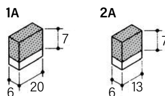
鑽石齒塊尺寸 / The dimensions of diamond tips
